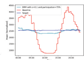
FIGURE 9. Results for the substation 34 for \epsilon = 0.1 and 75% participation. This specific substation had 70.52% participation.
