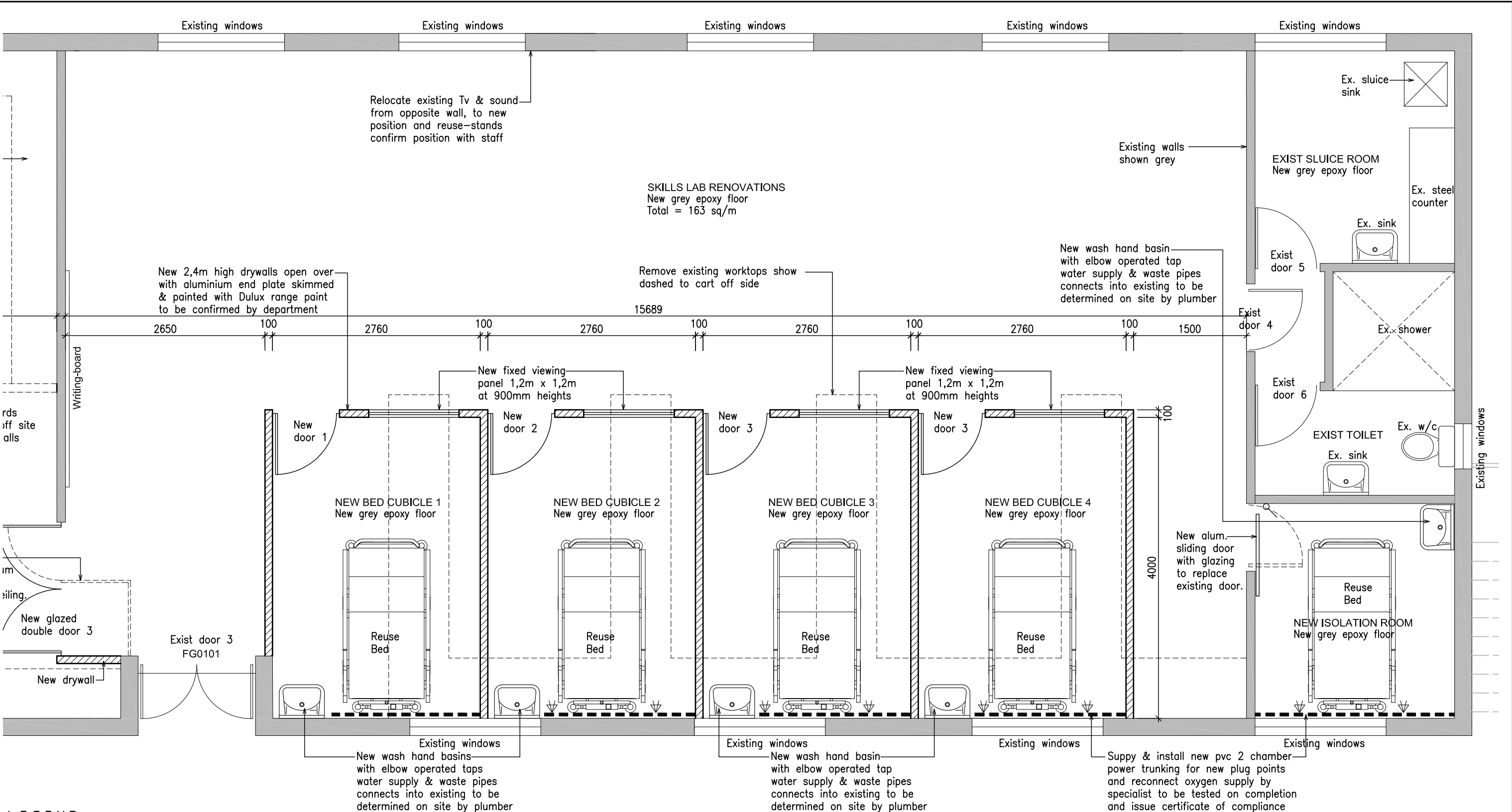
PART FIRST FLOOR PLAN - SKILLS LAB 1 IN 50
